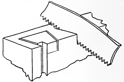
FIG. 432. SAWING TO KNIFE LINE.
